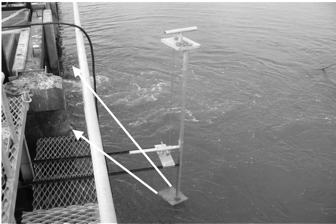
Figure 5. The DIDSON unit at the Murray mouth barrages. Arrows depict range of the beams. The unit was located to obtain an indication of fish behaviour outside the fishway entrance.
